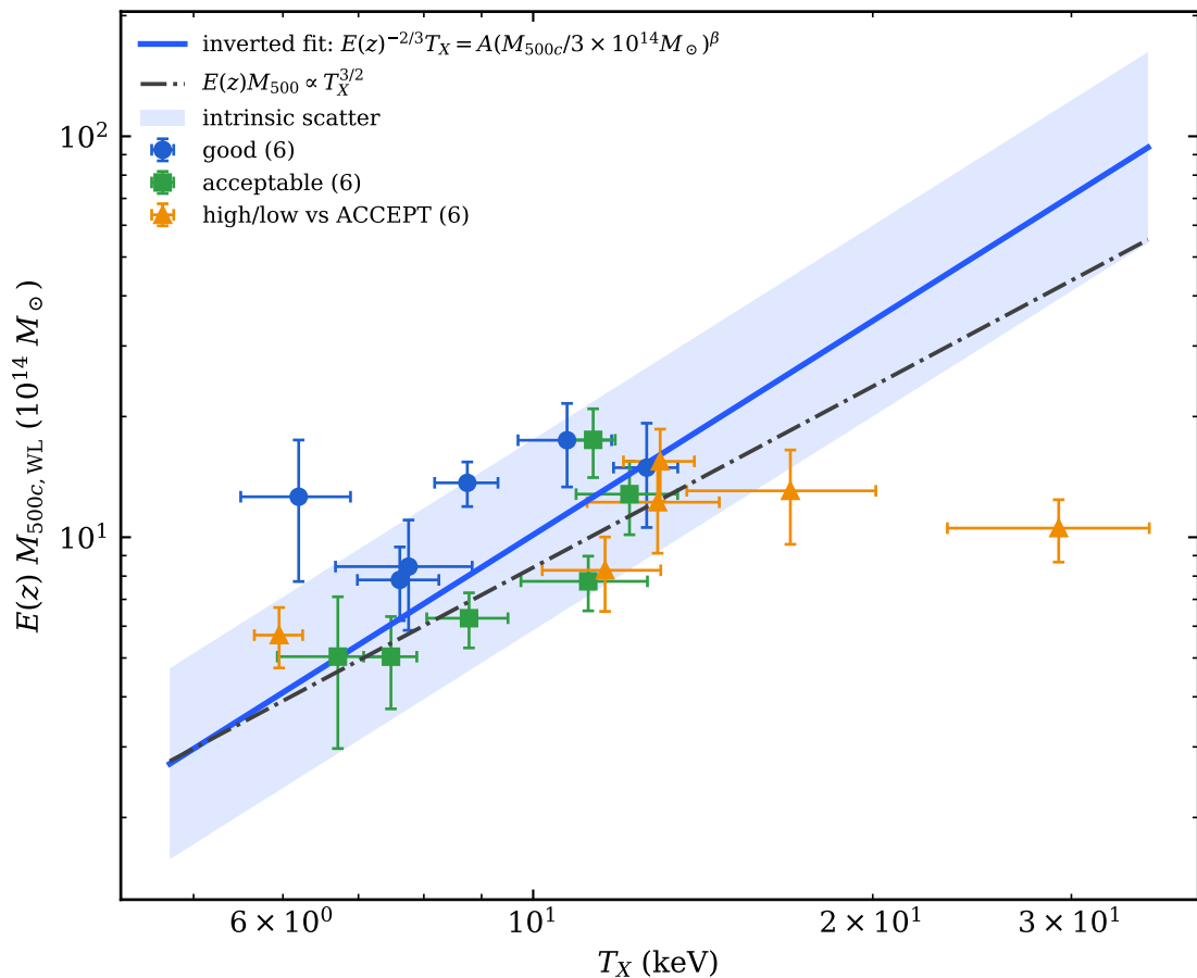
Literature-style M_{500c} - T_X (excluding bad/failed fits)
