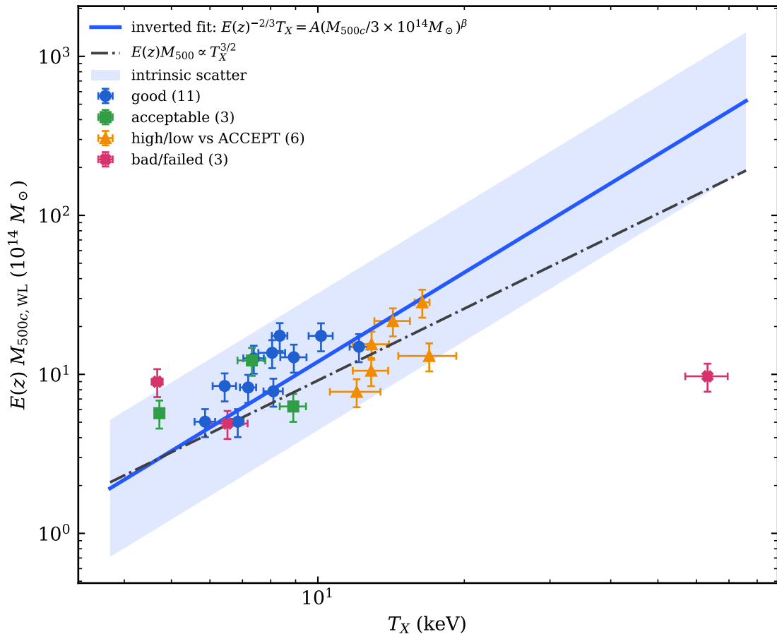
Literature-style M_{500c} - T_X (all fitted clusters)
