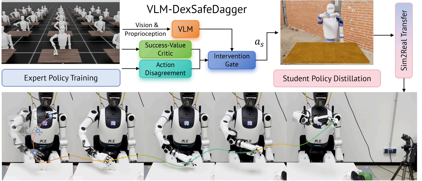
Fig. 1: VLM-DexSafeDagger overview. We propose a teacher-intervened online distillation pipeline that condenses teacher skills into a deployable RGB-based student policy. The unsafe exploration rate is substantially suppressed in the early training phase via a proposed VLM-guided intervention policy that combines teacher–student action disagreement with a Bellman success-value critic trained on safe-lift-success labels, while a vision-language model maintains an evolving, safety-aware understanding of the scene and periodically adjusts the intervention policy during online distillation.
