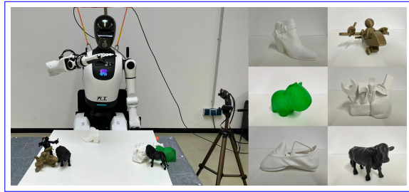
Fig. 5: Real-world experimental setup and test objects. Left: the single-arm manipulation platform used for deployment and evaluation. Right: examples of the physical objects used in the real-world lift experiments.
