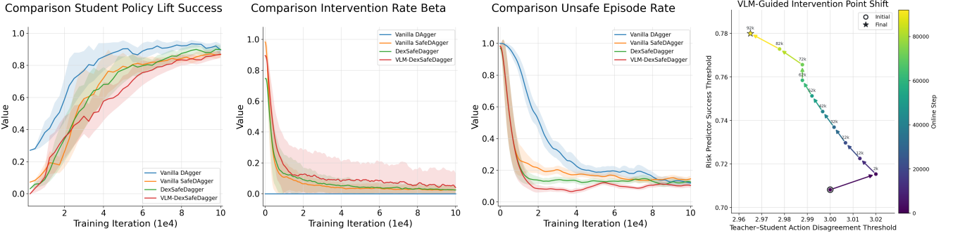
Fig. 3: Ablation studies. The first three panels compare four distillation variants in terms of student lift success, teacher intervention rate \beta , and unsafe episode rate, respectively, all plotted over training iterations. The rightmost panel shows the VLM-guided trajectory of the intervention operating point over online training. Shaded regions indicate variability across runs (mean \pm std). Curves correspond to vanilla DAgger (blue), vanilla SafeDagger (orange), DexSafeDagger (green), and VLM-DexSafeDagger (red).
