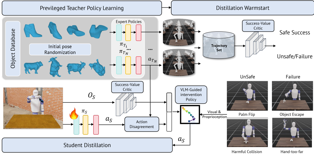
Fig. 2: Overview of the VLM-DexSafeDagger teacher-student learning pipeline. A privileged reinforcement learning teacher is trained in simulation and subsequently distilled into an RGB-based visuomotor policy for real-world deployment. A vision-language model periodically proposes a displacement of the intervention policy’s operating point; deterministic clipping and smoothing constrain the resulting policy update.
