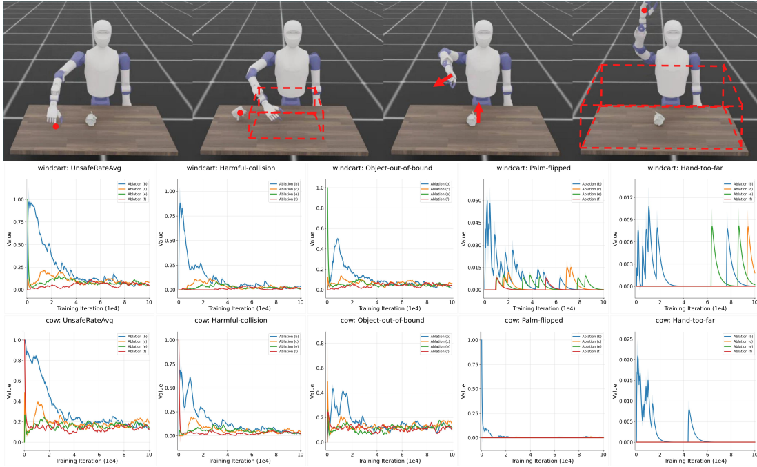
Fig. 4: Per-object failure-mode decomposition during online distillation. For WindCart and Cow, we show the aggregate unsafe-episode rate and its breakdown into harmful collision, object escape, palm flip, and hand-too-far over training; lower is better. Blue: Vanilla DAgger [10]; orange: Vanilla SafeDagger [12]; green: DexSafeDagger; red: VLM-DexSafeDagger.
