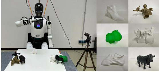
Fig. 5: Real-world setup and test objects. Left: Tiangong 2 Pro with an InspireHand RH56DfX and an external stereo camera. Right: test objects.
