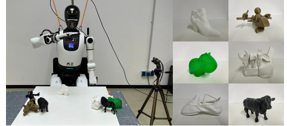
Fig. 5: Real-world experimental setup and test objects. Left: the single-arm manipulation platform used for deployment and evaluation. Right: examples of the physical objects used in the real-world lift experiments.
