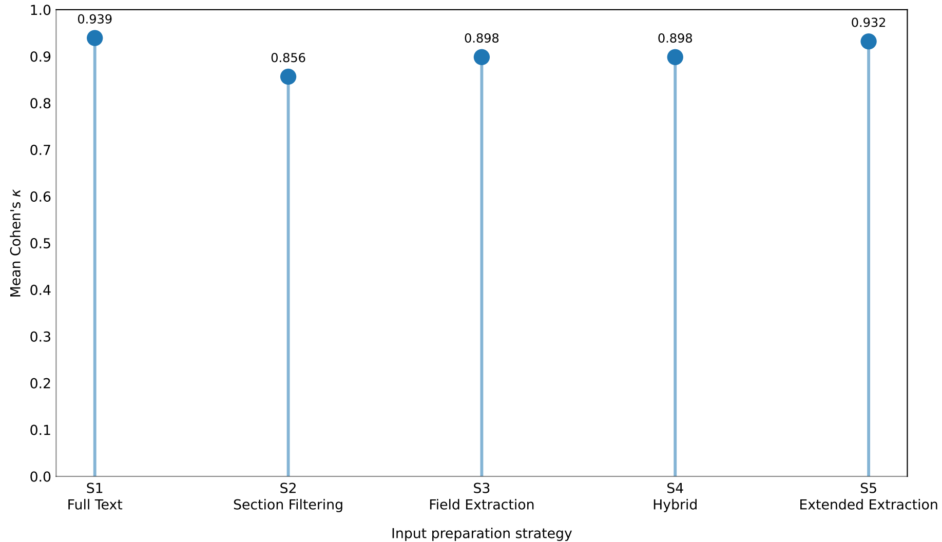
Output Consistency Across Repeated Runs
