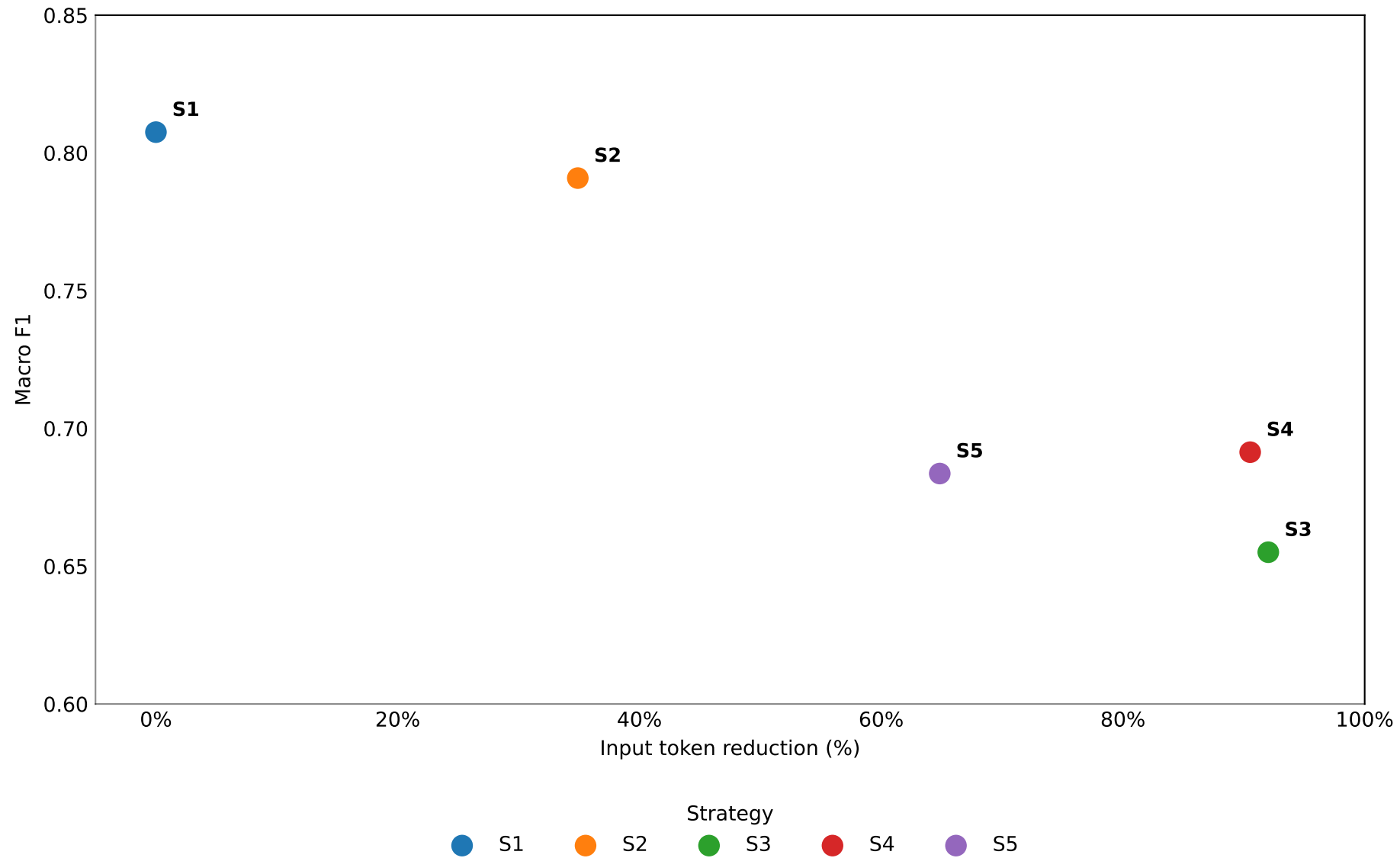
Quality-Efficiency Trade-off Across Input Strategies
