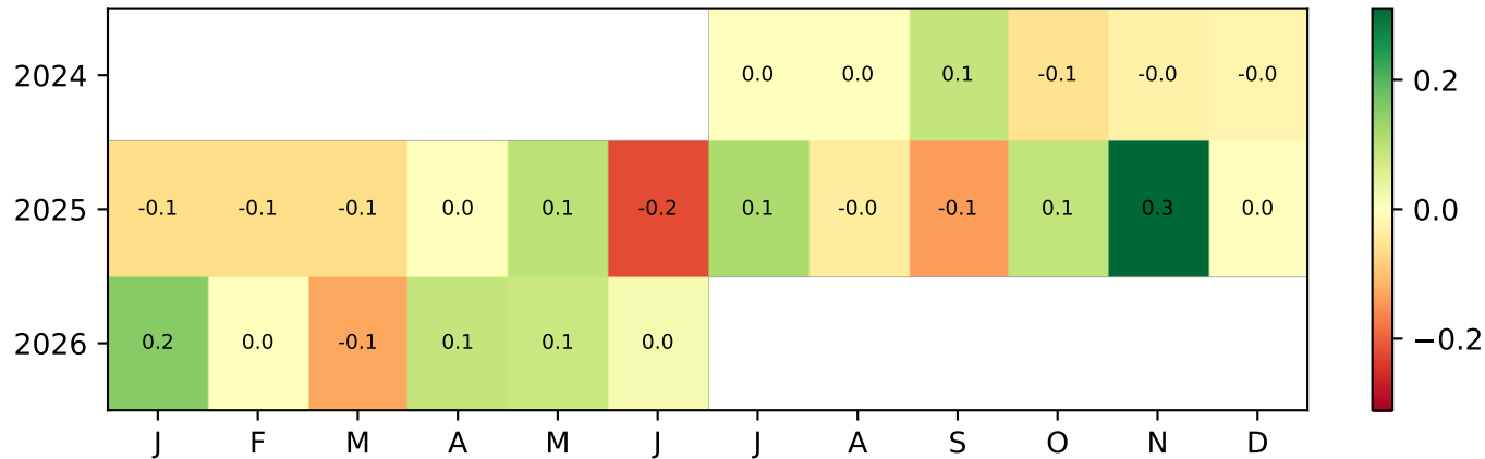
Monthly returns (%)
