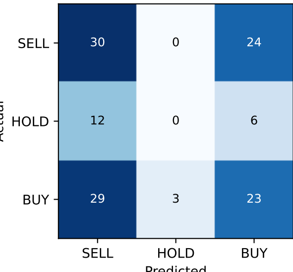
Confusion matrix (acc 0.417)
