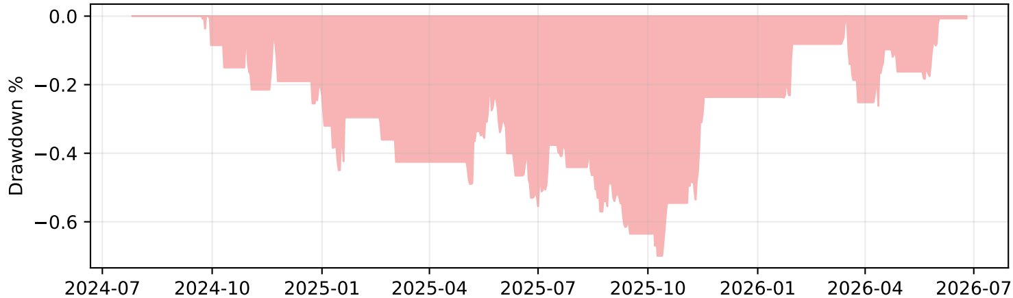
Underwater drawdown (%)
