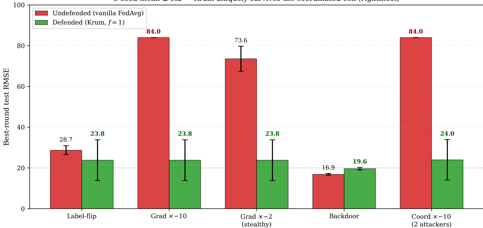
Defense recovery: vanilla FedAvg vs Krum ( f=1 ) under each attack 5-seed mean \pm std --- Krum uniquely survives the coordinated cell (rightmost)
