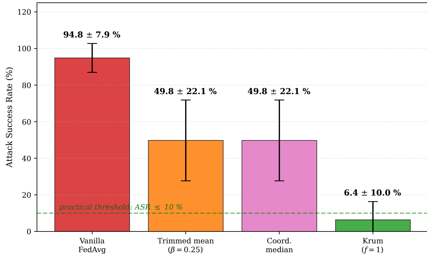
Axis 2 --- sensor-value backdoor: Attack Success Rate by aggregator 5-seed mean \pm std, seeds \in \{42, 43, 44, 45, 46\}
