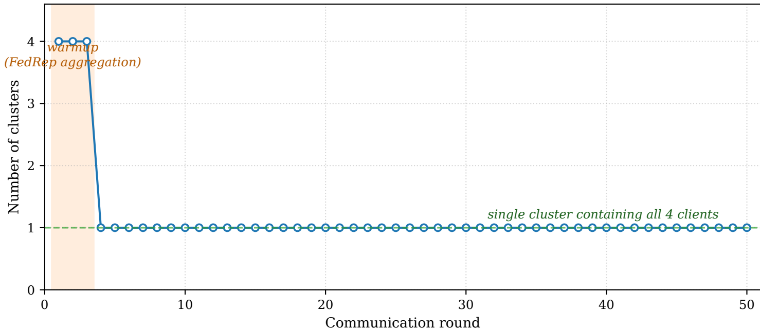
FedCCFA cluster structure across communication rounds After warmup the similarity threshold \tau = 0.5 never partitions the federation
