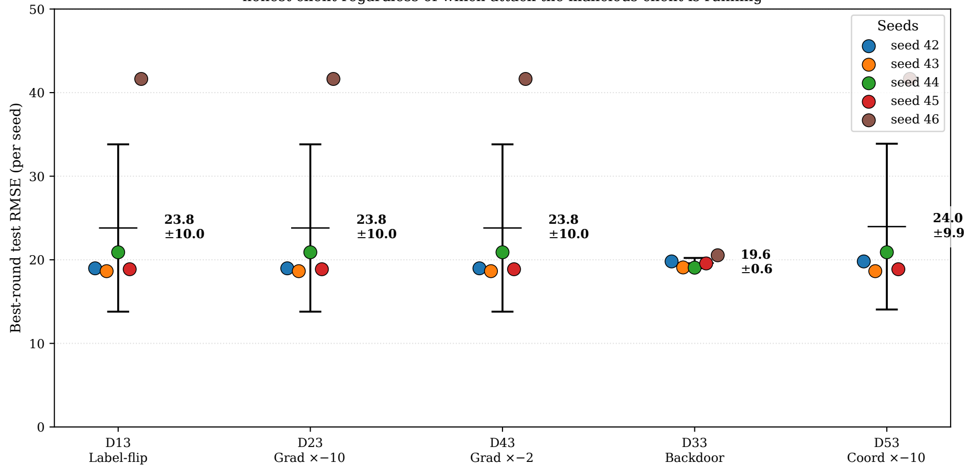
Krum-defense per-seed RMSE across 5 attack cells The 3 leftmost cells share identical (mean, std) --- Krum's argmin selects the same honest client regardless of which attack the malicious client is running
