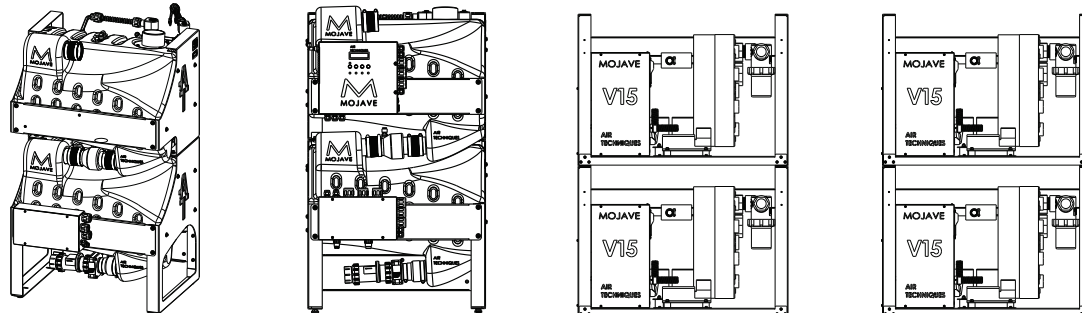
4V15 System Installation Two Side by Side Stacks of Two V15 Pumps with CT12 and CT34 Tanks on the Side
