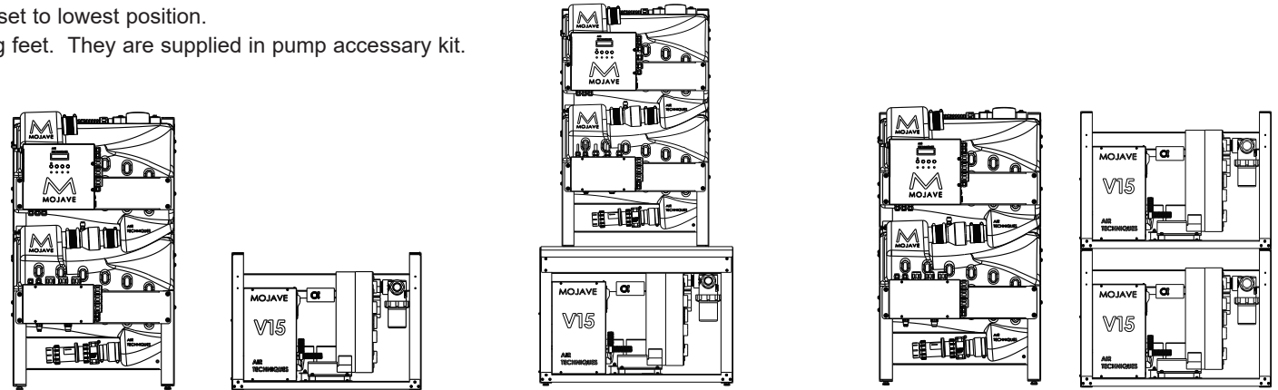
Stacked V15 System Installation: One CT12 Tank above One V15 Pump (See note.)
