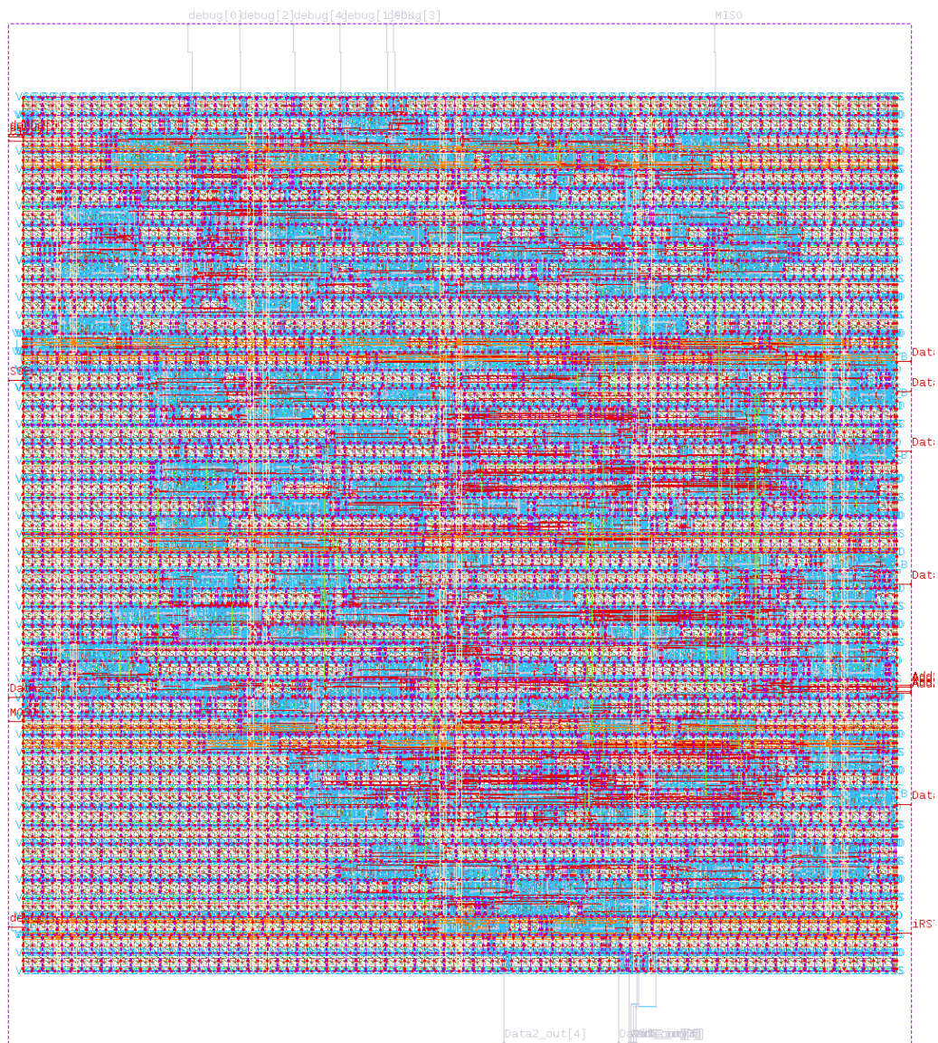
Mode-0 variant, 3.3 V sg13g2_stdcell_hv — final routed layout, 354.38 \mu\text{m} \times 399.98 \mu\text{m} . Note the 7.14 \mu\text{m} rows and coarser fabric of the thick-oxide cells.
