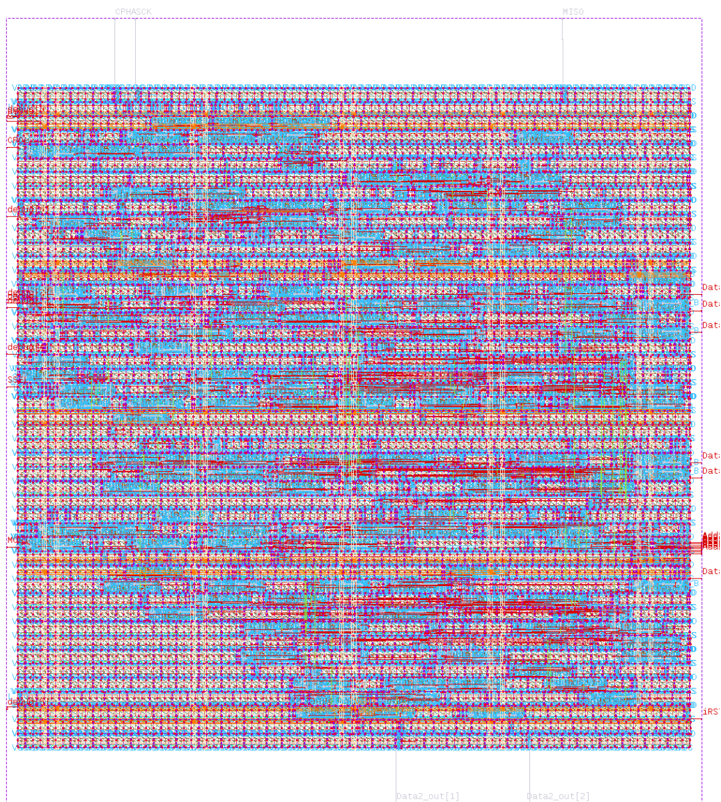
All-modes variant, 3.3 V sg13g2_stdcell_hv — final routed layout, 354.01 \mu\text{m} \times 399.61 \mu\text{m}
