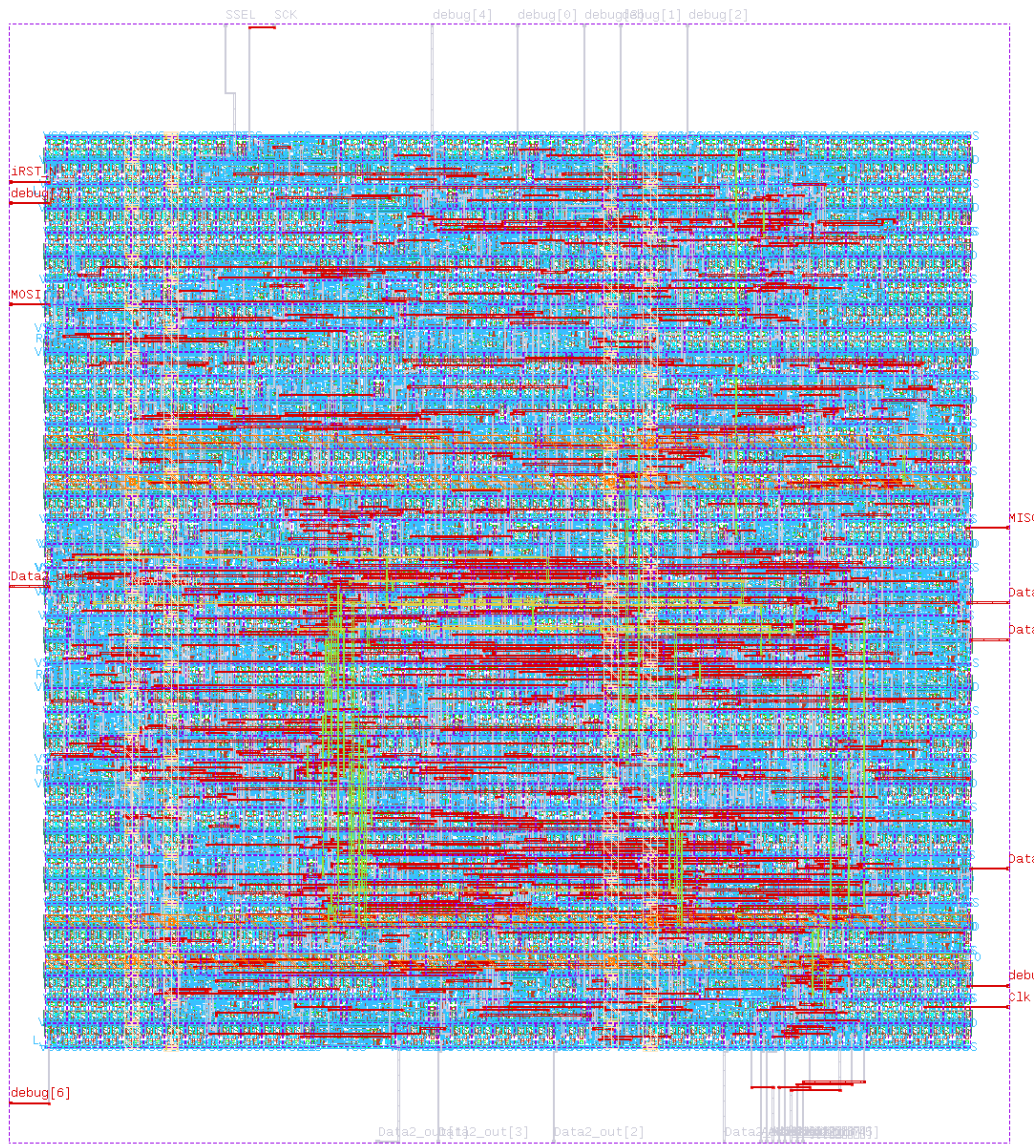
Mode-0 variant, 1.2 V sg13g2_stdcell — final routed layout, 157.78 \mu\text{m} \times 176.50 \mu\text{m} (KLayout render, IHP layer styles)
