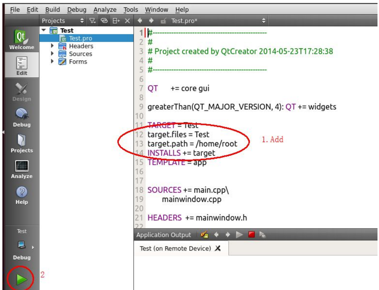
Figure 820: Test.pro file
