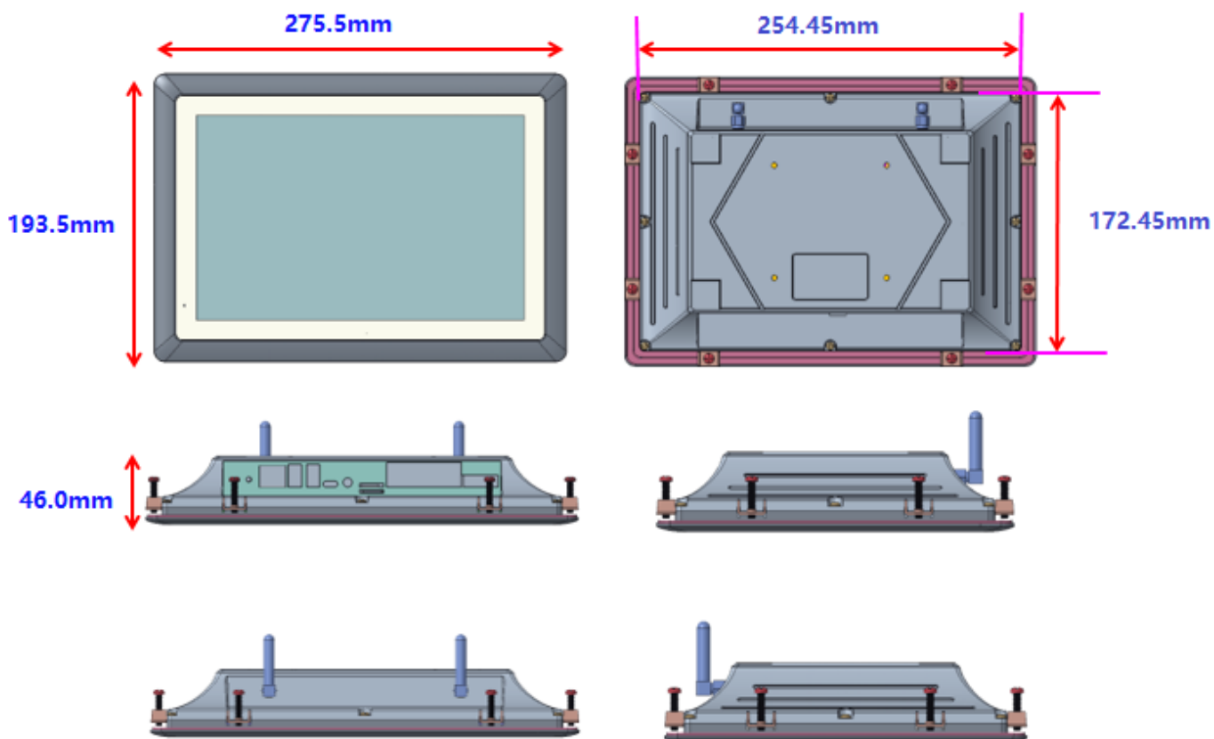
Panel mounting (PPC-RK3576-101)
