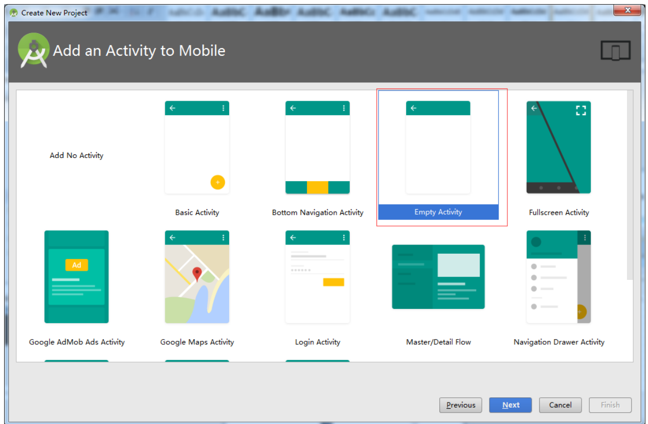
Figure 210: Add Activity
