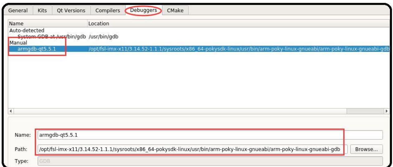
Figure 379: Debuggers
