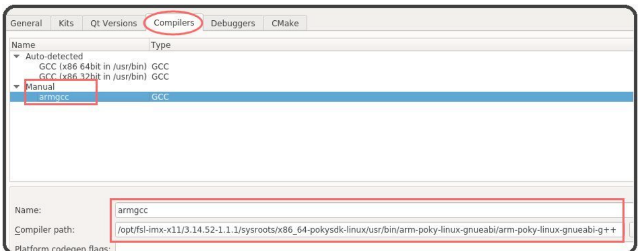
Figure 380: Compilers
