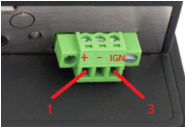
Power Input
