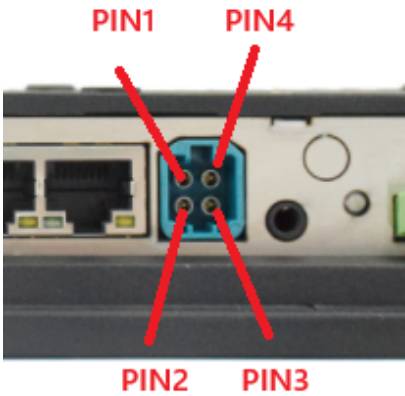
Fakra-Mini automotive Connectors
