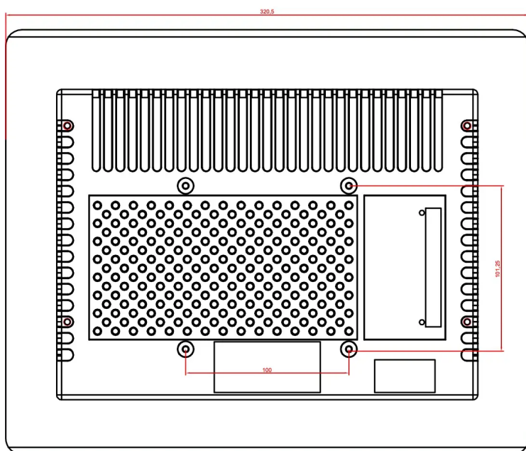
Figure 917: CS10768RA4121P Technical Drawing
