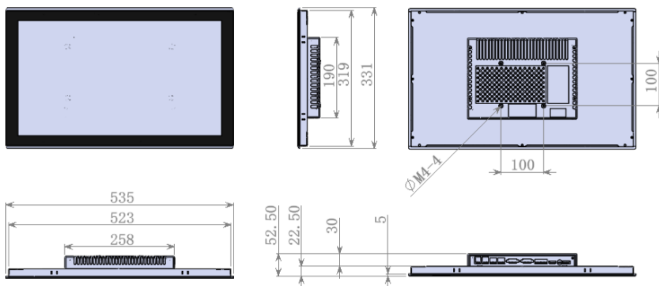
Dimensions (PPC-RK3576-215)
