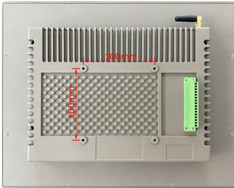
Figure 568: VESA Mounting-1
