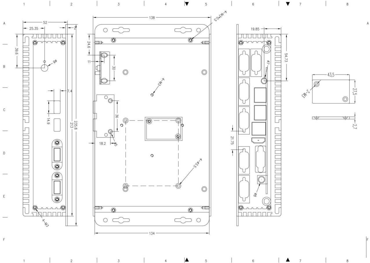
CS86-BOX-5500U Technical Drawing
