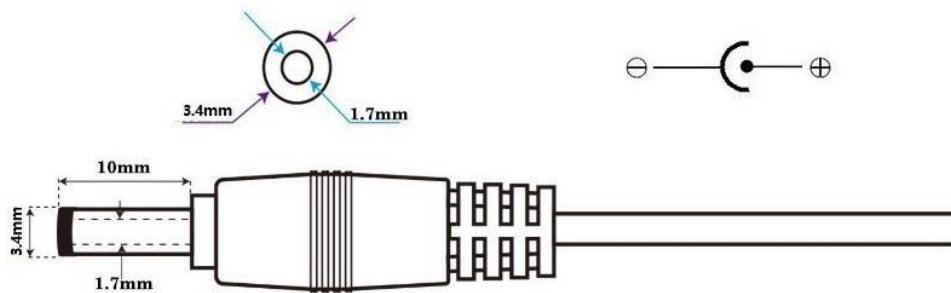
Power Connector
