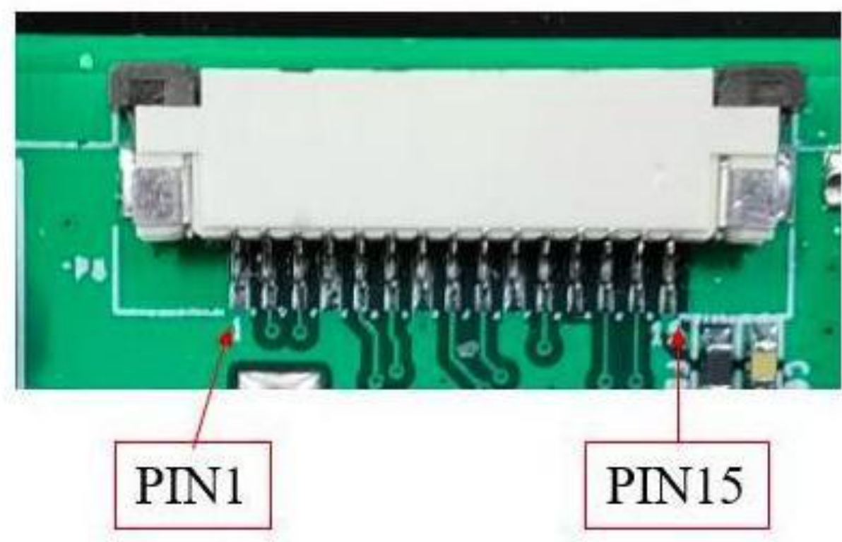
Camera Connector
