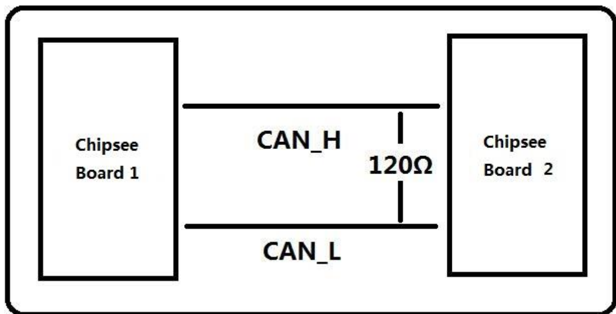
Figure 1018: Connecting CAN
