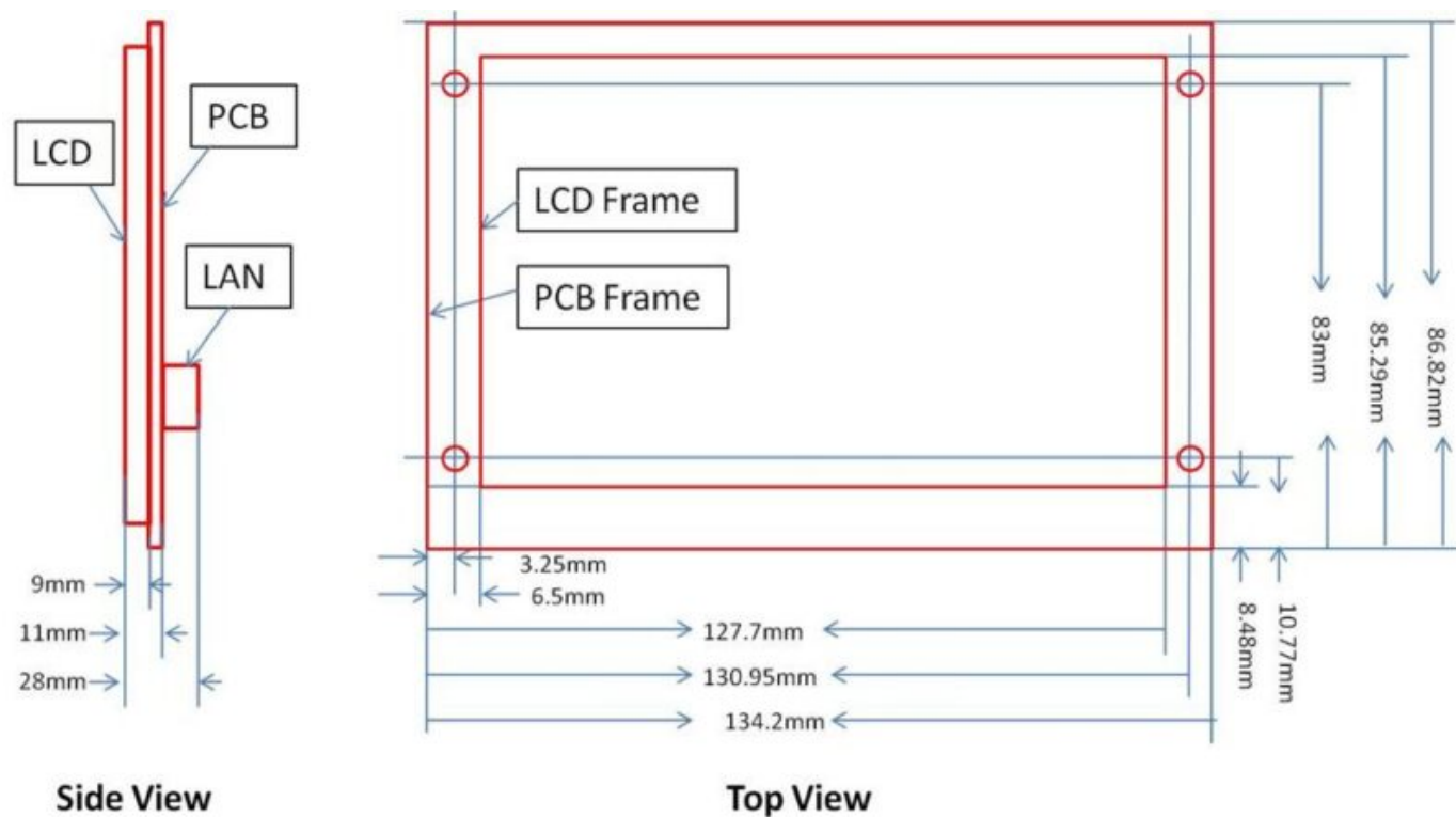
Figure 683: EPC-A8-050-C Technical Drawing
