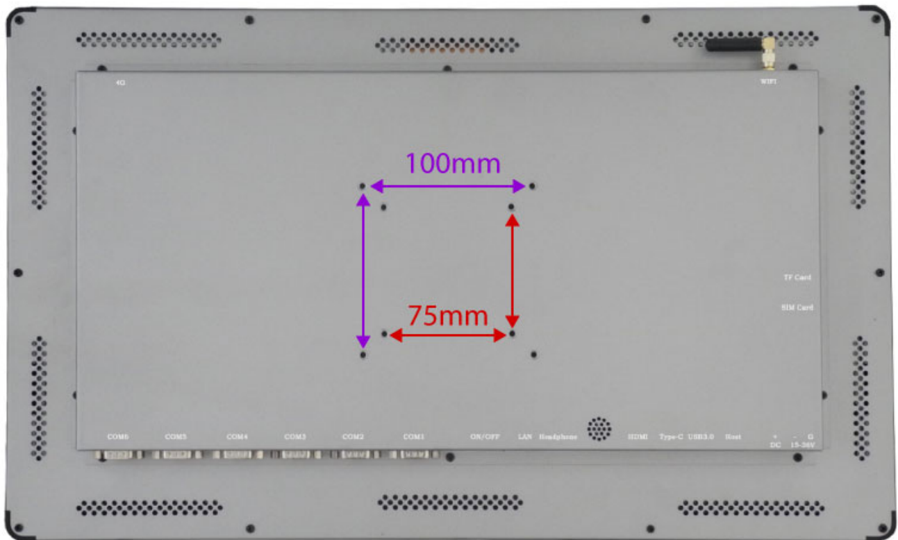
Figure 600: Mounting Method
