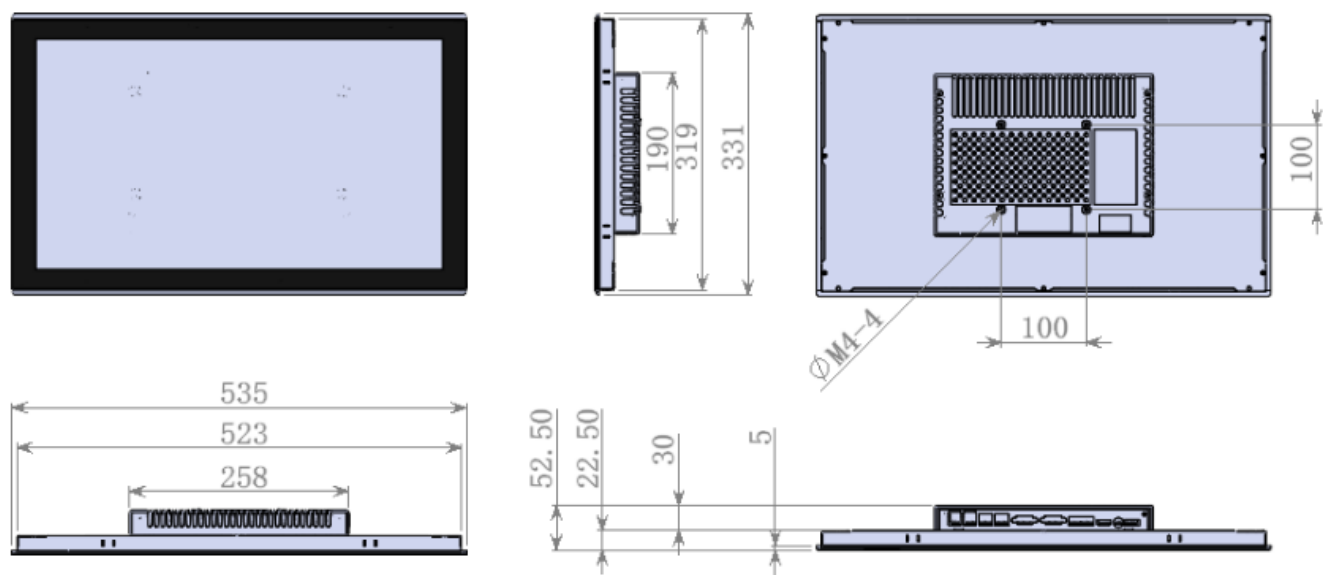
Dimensions (PPC-RK3576-215)
