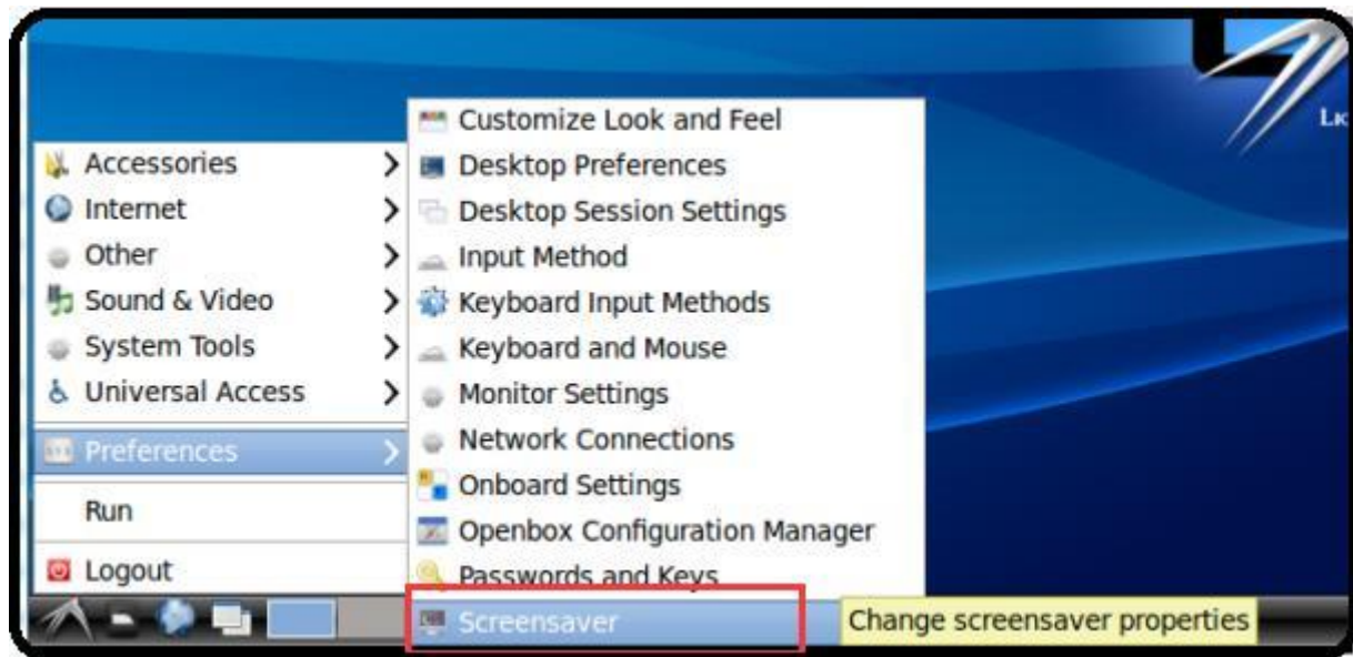
Figure 329: Screensaver
