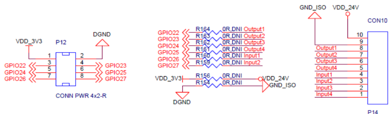
CPU GPIO Reduced Schematic
