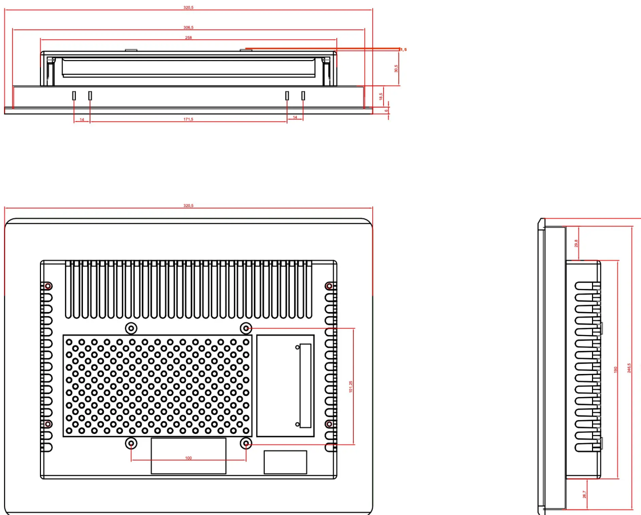
Figure 917: CS10768RA4121P Technical Drawing
