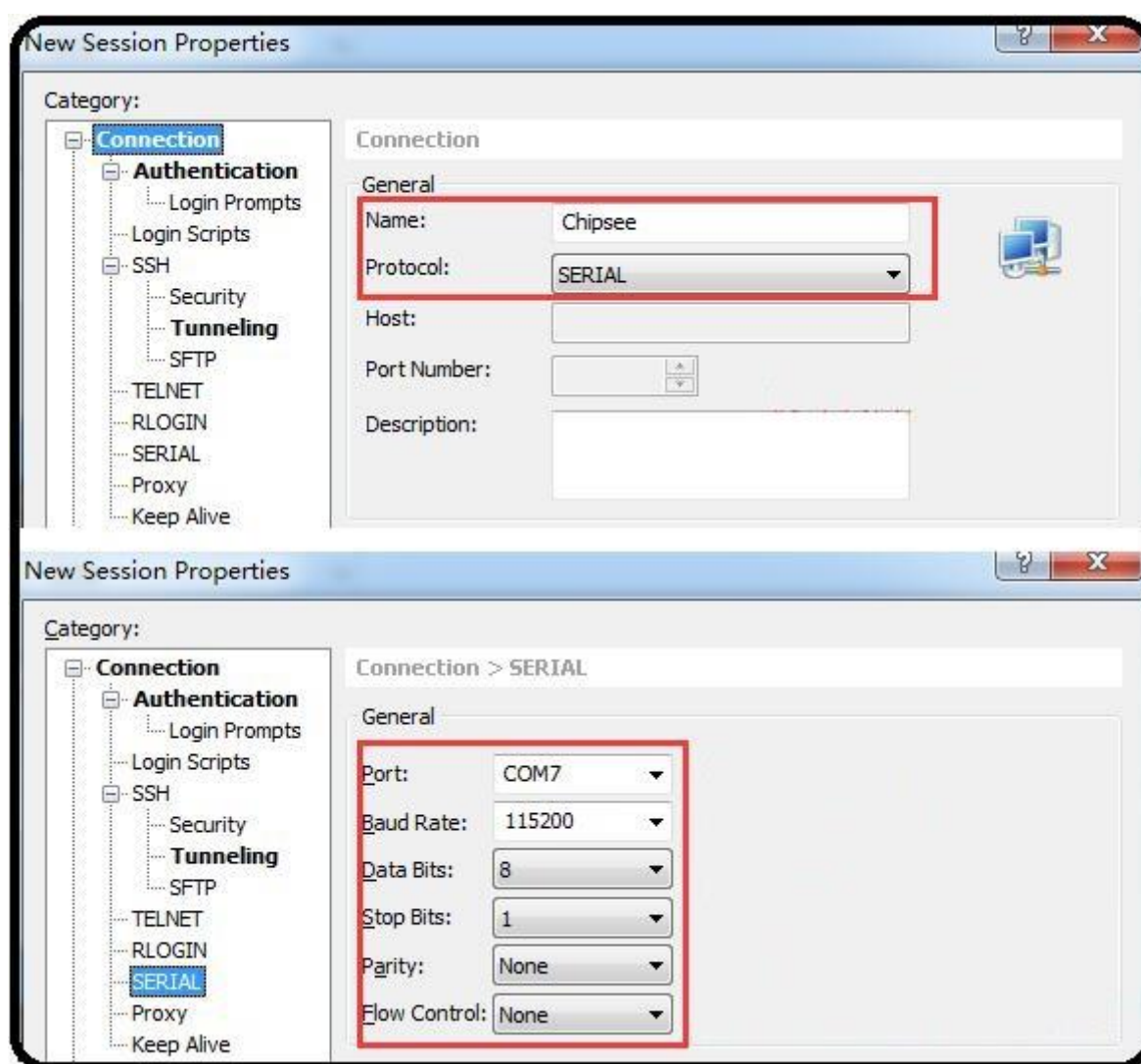
Figure 1009: Session Properties
