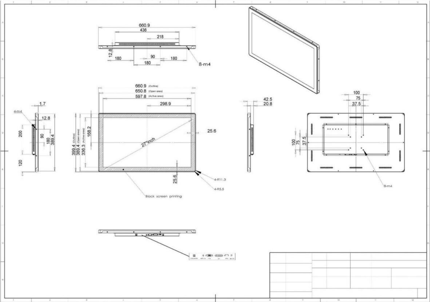
Figure 1030: Technical Drawing
