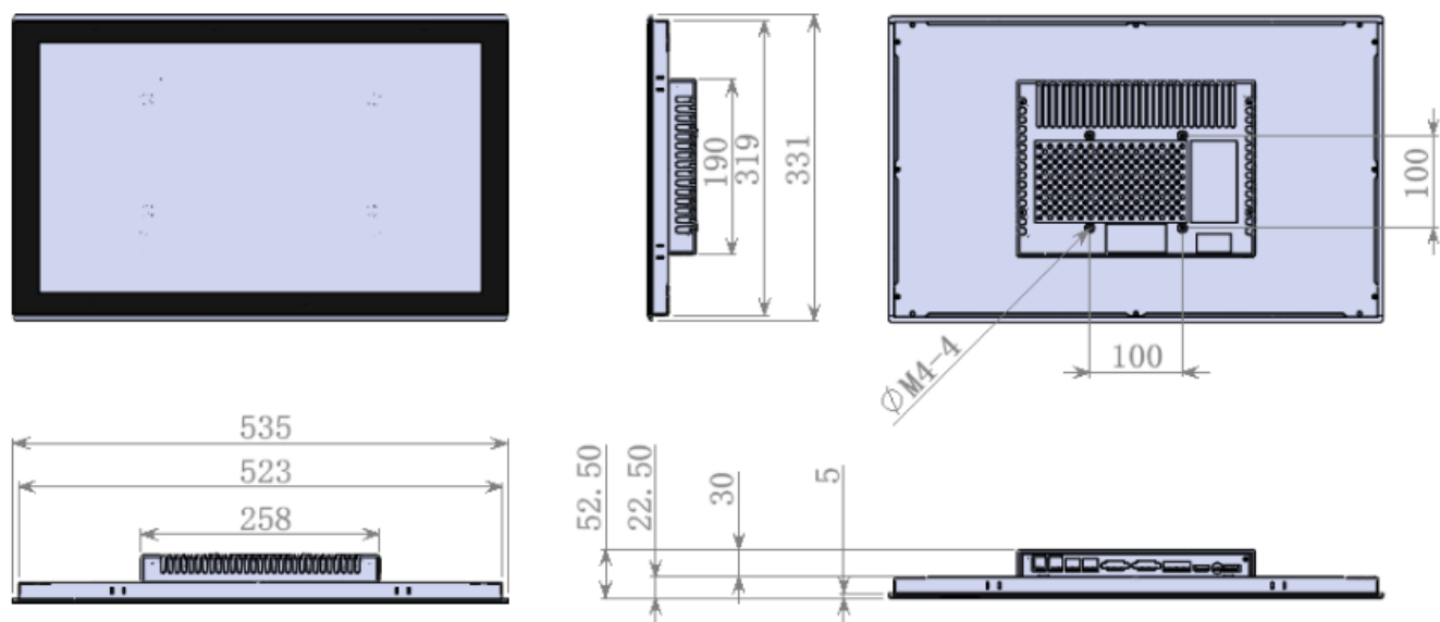
Dimensions (PPC-RK3576-215)
