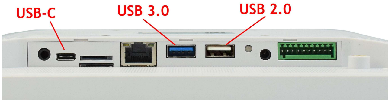
USB3.0 HOST and Type-C Connectors
