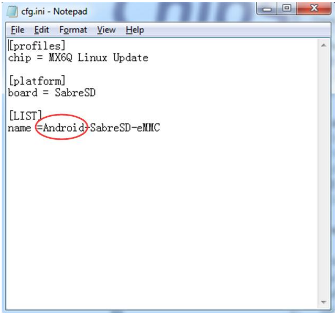
Figure 131: Cfg.ini file
