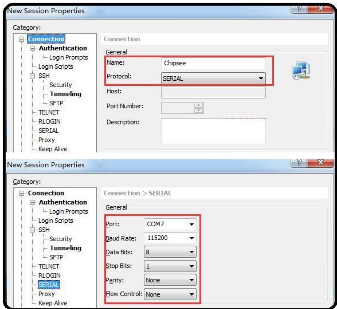
Figure 292: Session Properties
