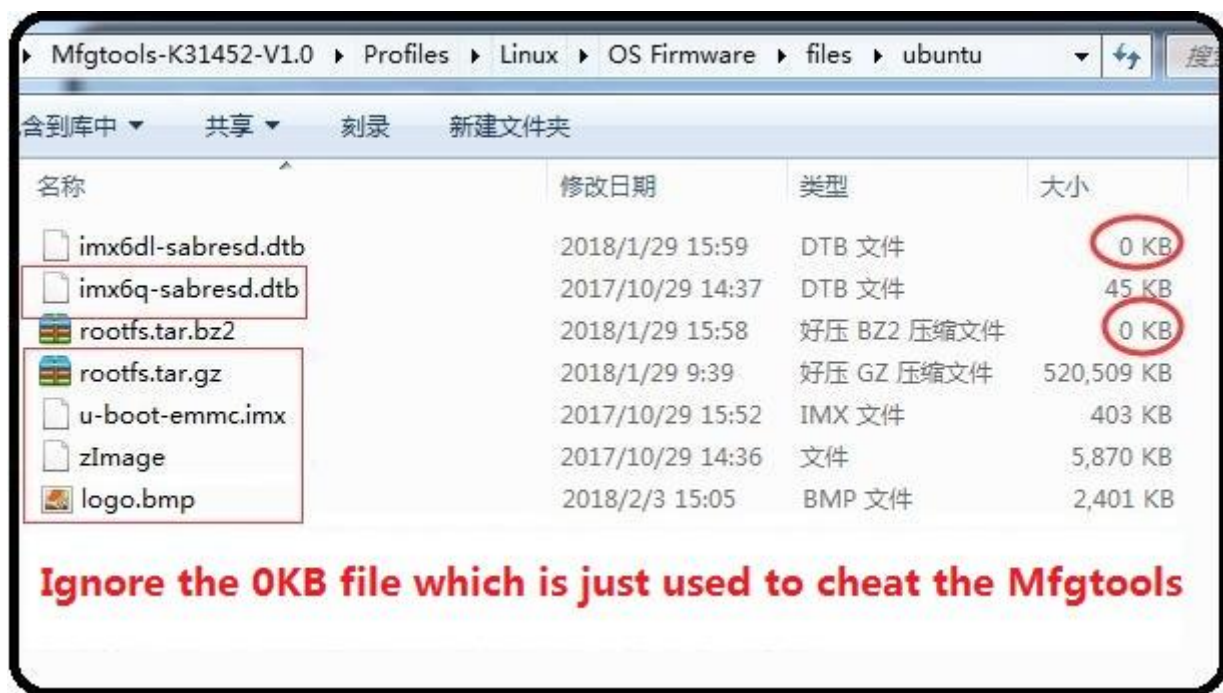
Figure 303: Prepare Images
