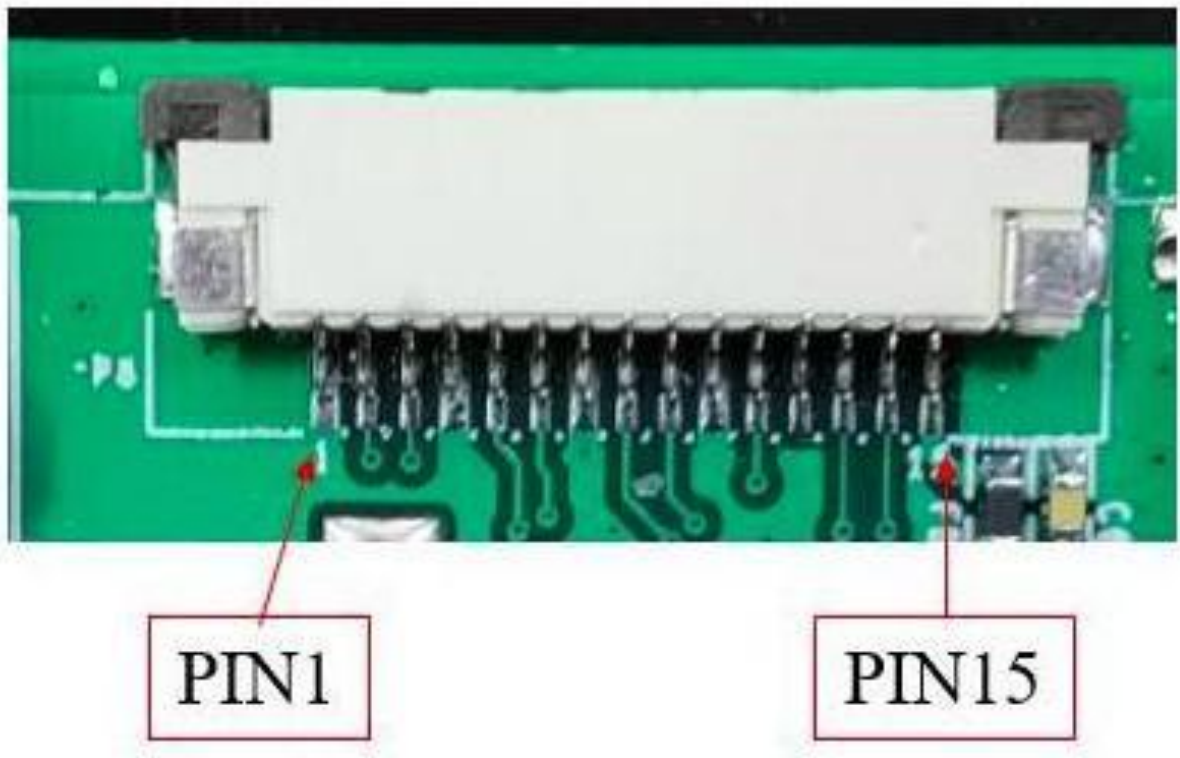
Camera Connector
