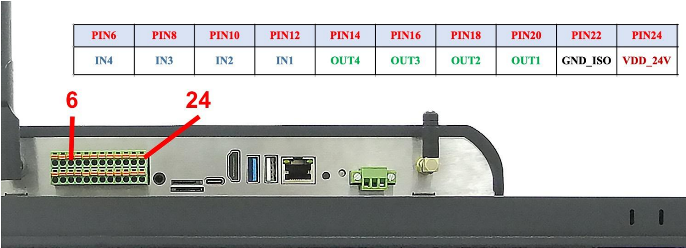
GPIO Terminal
