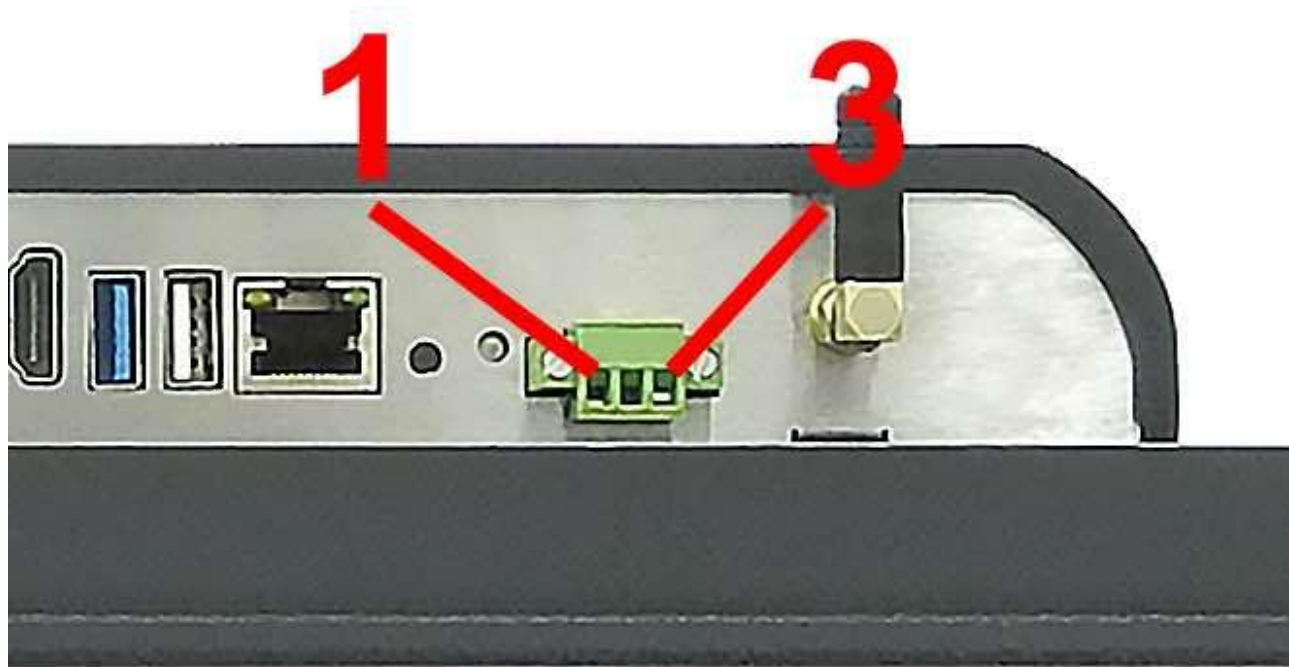
Power Input
