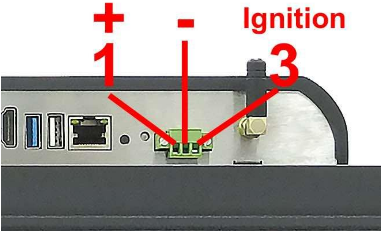
Power Input (with Ignition Signal)
