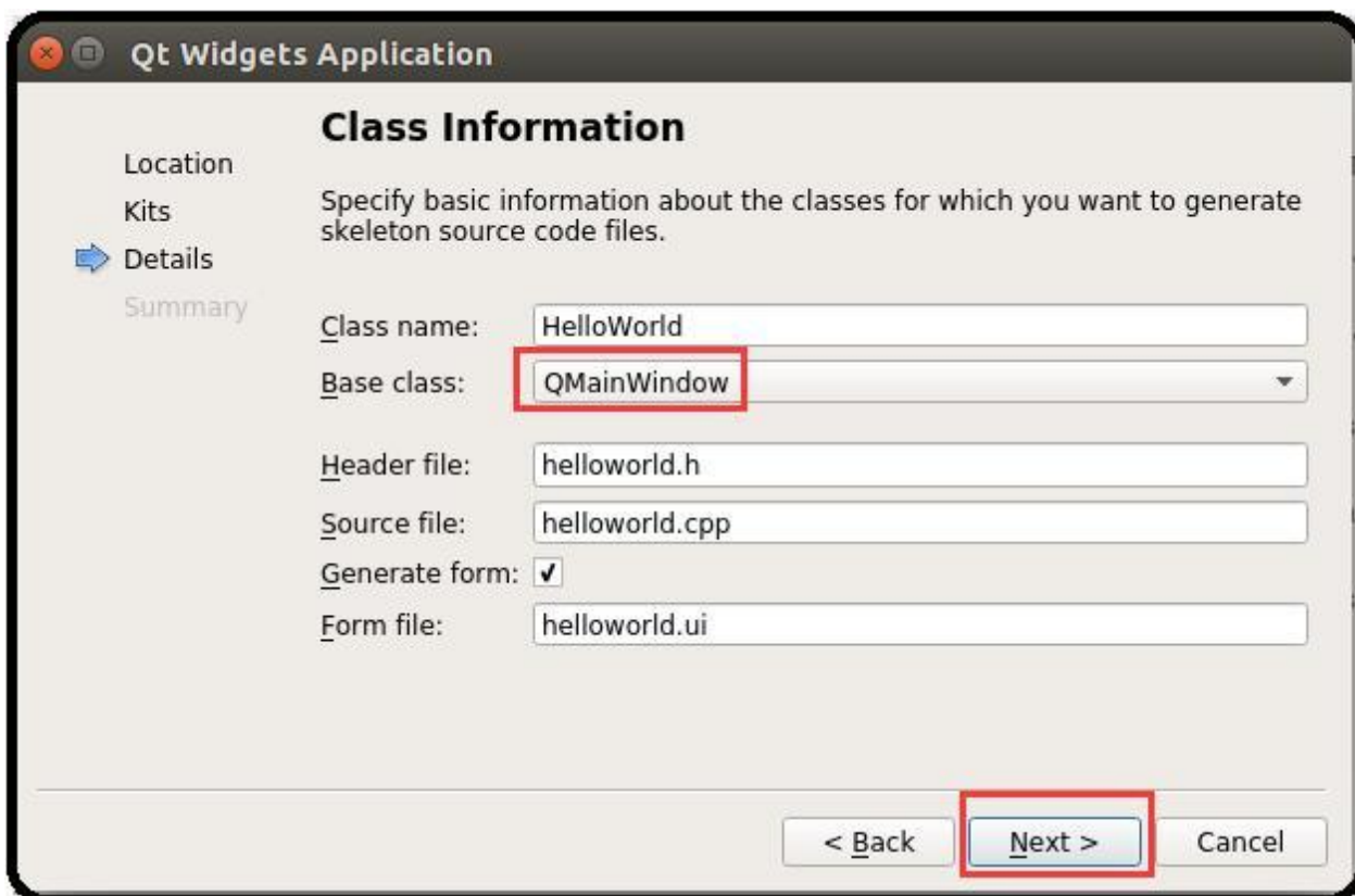
Figure 258: Base Class
