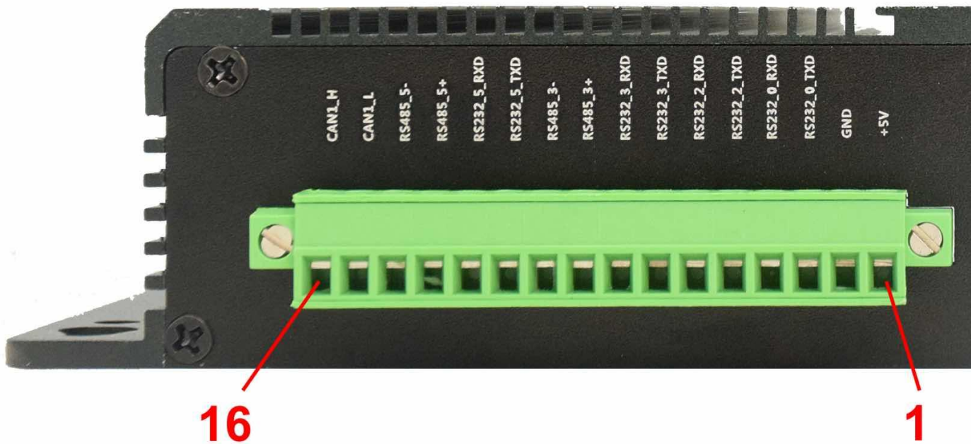
RS232-RS485-CAN on the CS-CM4-BOX Industrial PC
