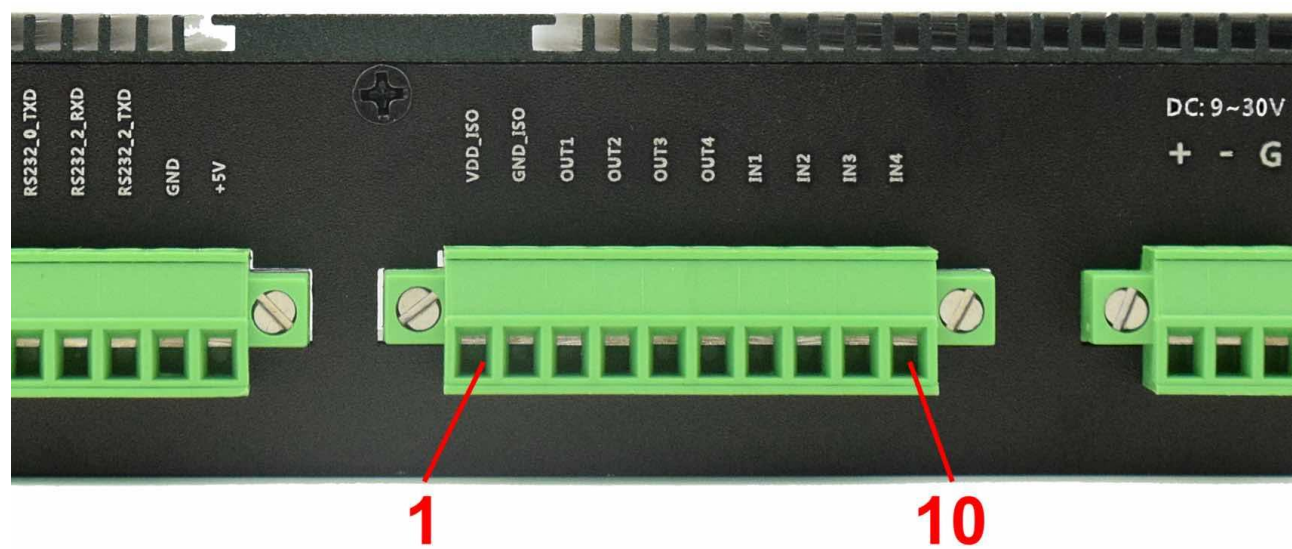
GPIO Terminal
