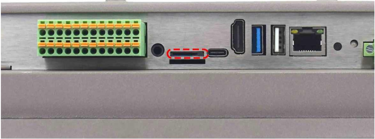
TF (micro SD) Card Slot
