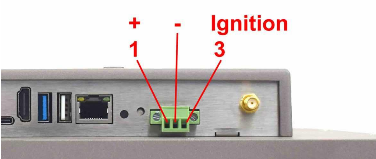
Power Input (with Ignition Signal)
