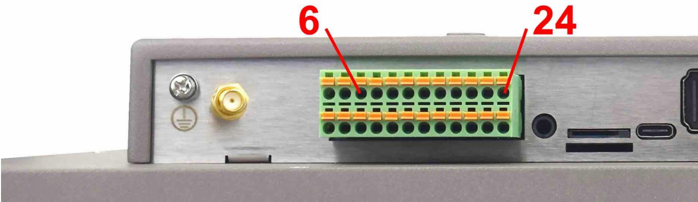
GPIO Terminal
