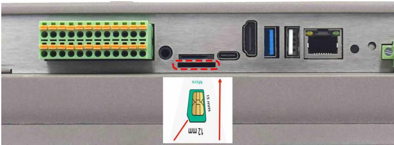
SIM Card Direction
