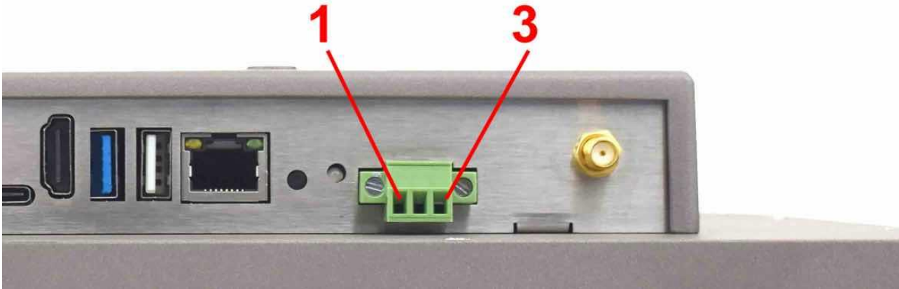
Power Input
