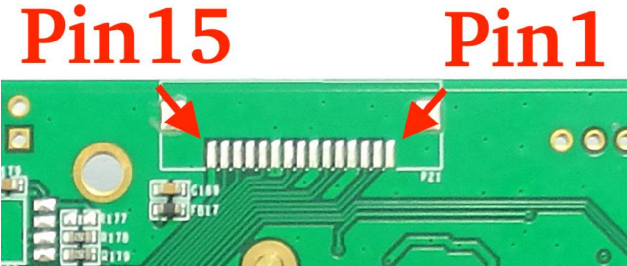
Camera Connector
