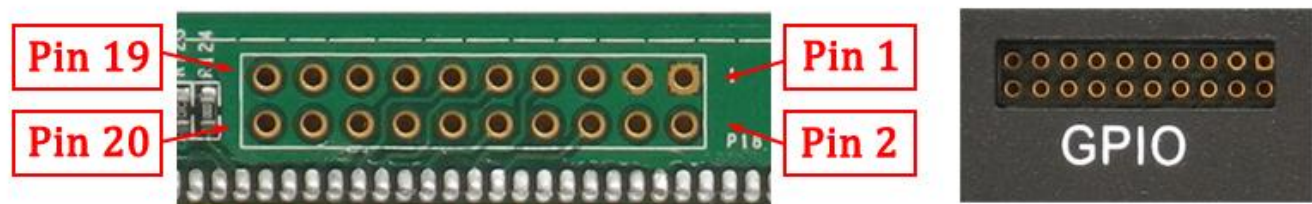
Figure 722: Expansion Port
