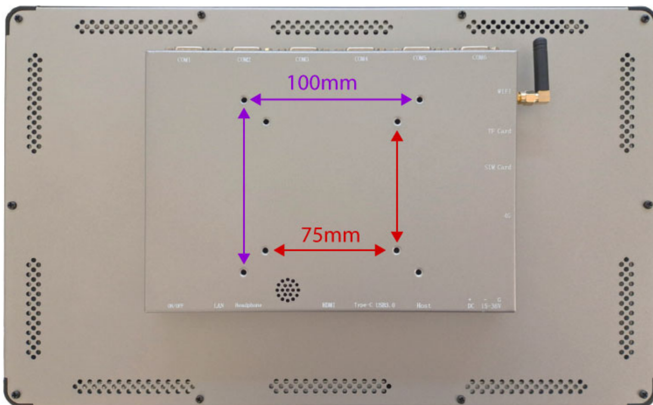
Figure 585: Mounting Method
