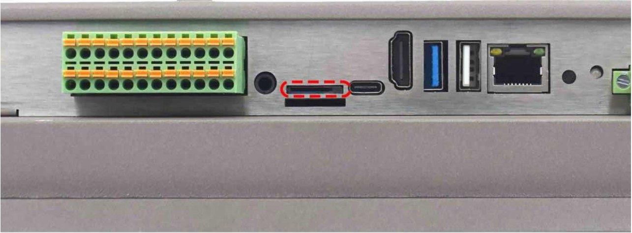
TF (micro SD) Card Slot
