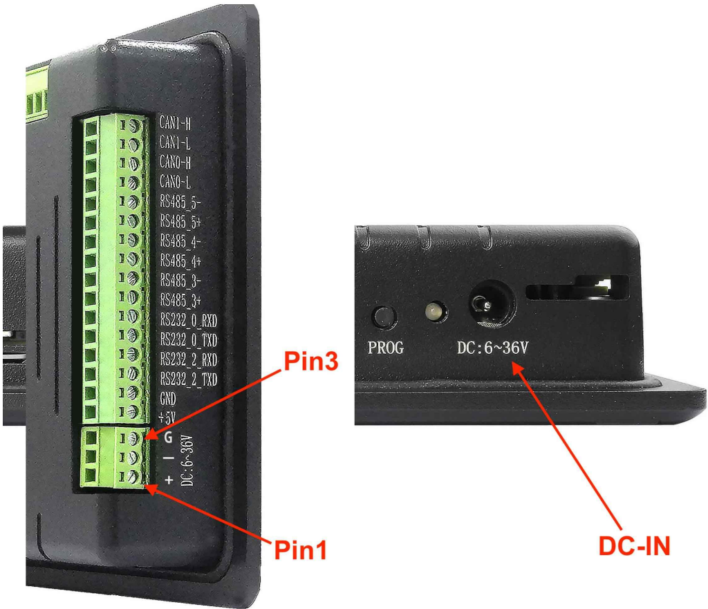
Power Input
