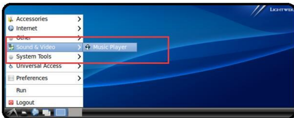
Figure 318: LXMusic
